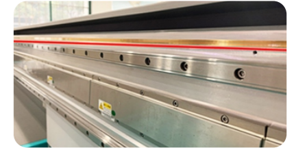
Metallic Optical Encoder Scale, which is oil resistant, stable in moving with ease of maintenance and accuracy of reading.
